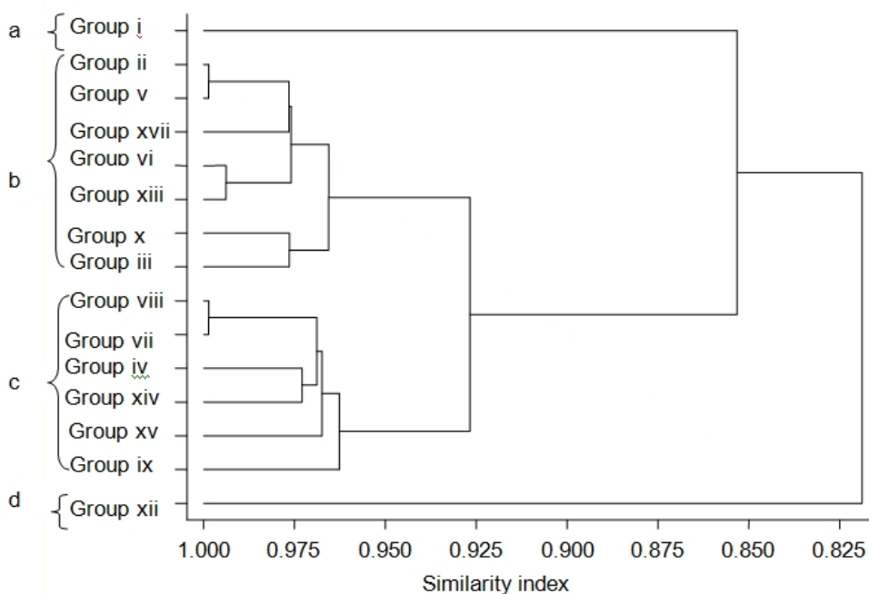
Fig. 5. Dendrogram showing morphological diversity of farm trapping rhizobia isolates from Lake Victoria Basin
