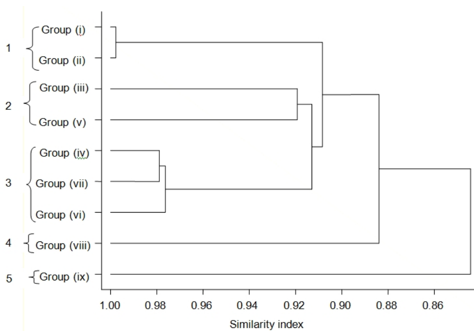
Fig. 4. Dendrogram showing morphological diversity of whole soil trapping rhizobia isolates from Lake Victoria Basin
