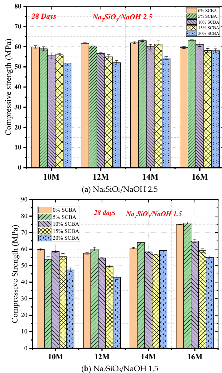
Figure 5. Effect of NaOH concentration in the compressive strength of FA-SCBA based GPC.
