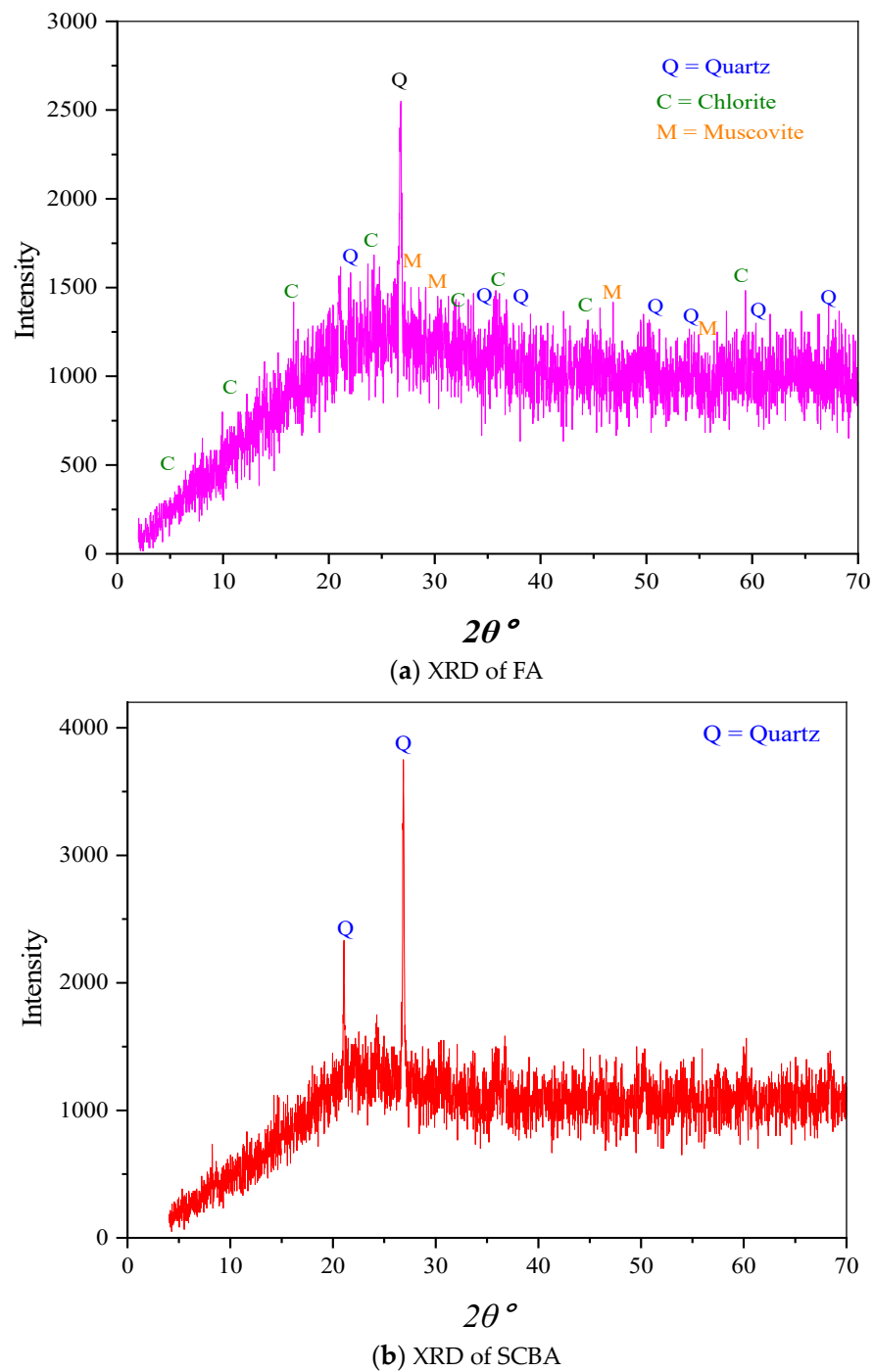
Figure 1. XRD of FA and SCBA.
