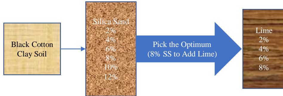
Fig. 1 Schematic layout of treatment of black cotton soil
