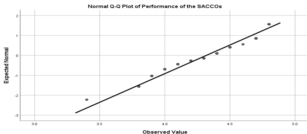
Figure 4. 6: Normal Q-Q plot of performance
